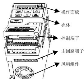
II 类外观 适用机型 DL100-2S0007(B)~DL100-2S0015(B) DL100-4T0007(B)~DL100-4T0015(B)
